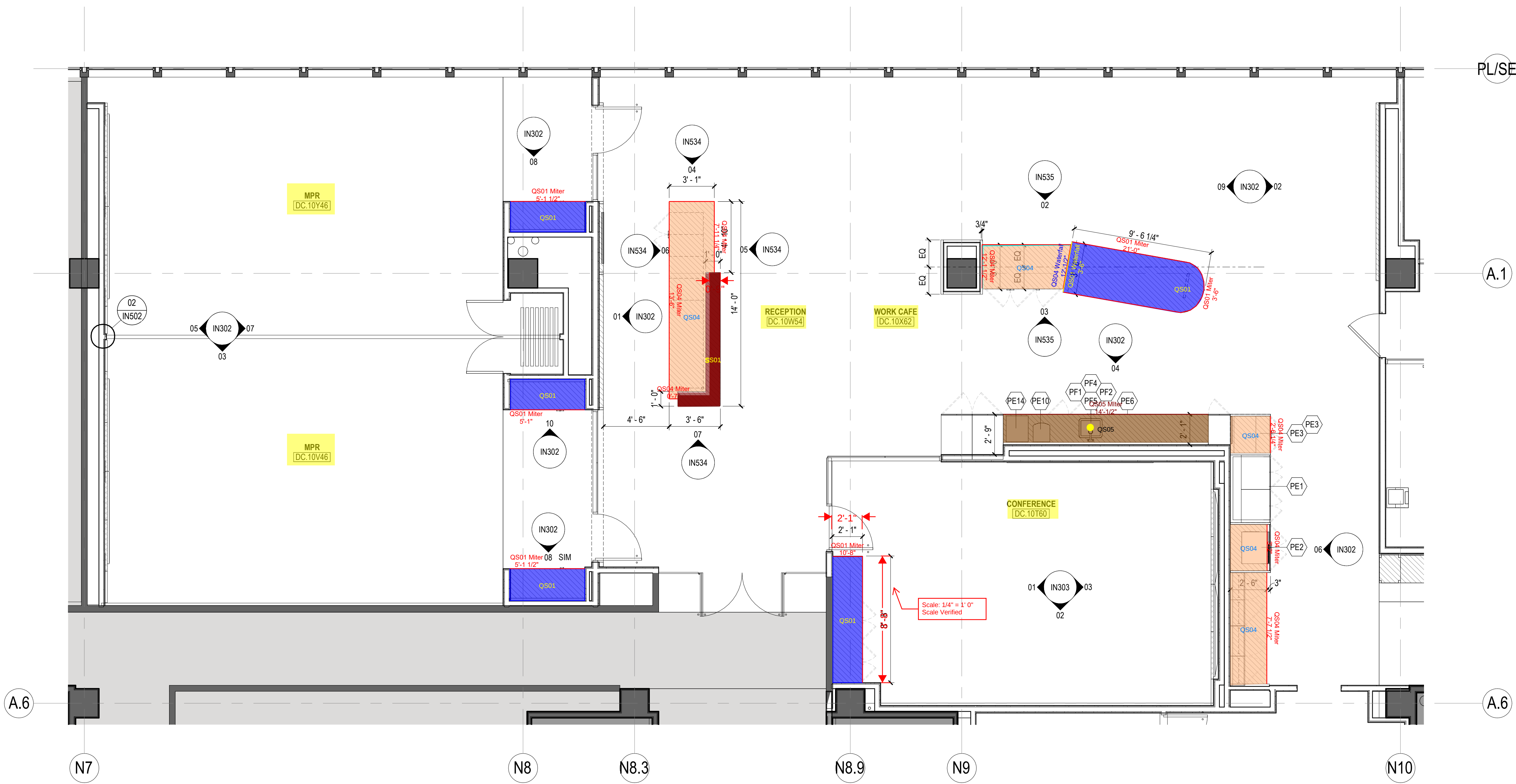
01 ENLARGED PLAN - RECEPTION SCALE: 1/4" = 1'-0"
